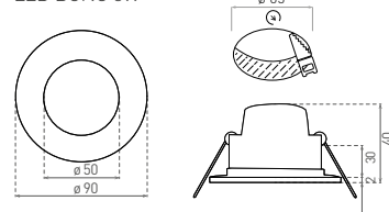
LED BONO 5W
