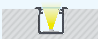
EN Installation instruction for recessed profile G with a BASIC cover.
